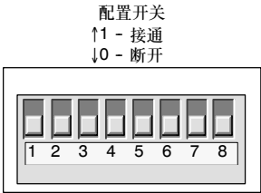
图A-24 EM231RTD模块的DIP开关
