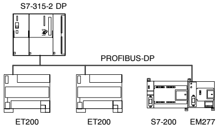
图7-17 S7-315-2DP网络
